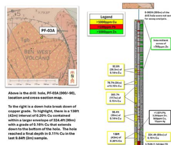
Drill Hole PF-03A Location and Cross Section Map
