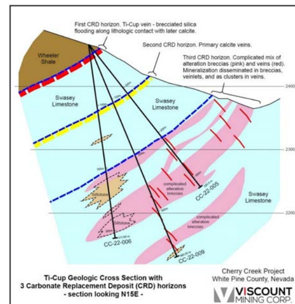
Ti-Cup CRD cross-section, Cherry Creek
